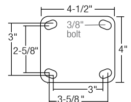
Top plate bolt hole pattern
